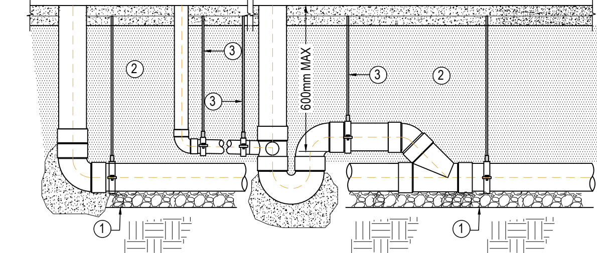
RECOMMENDED PIPE SUPPORT LOCATIONS ON "E" TYPE SOILS NOT TO SCALE
