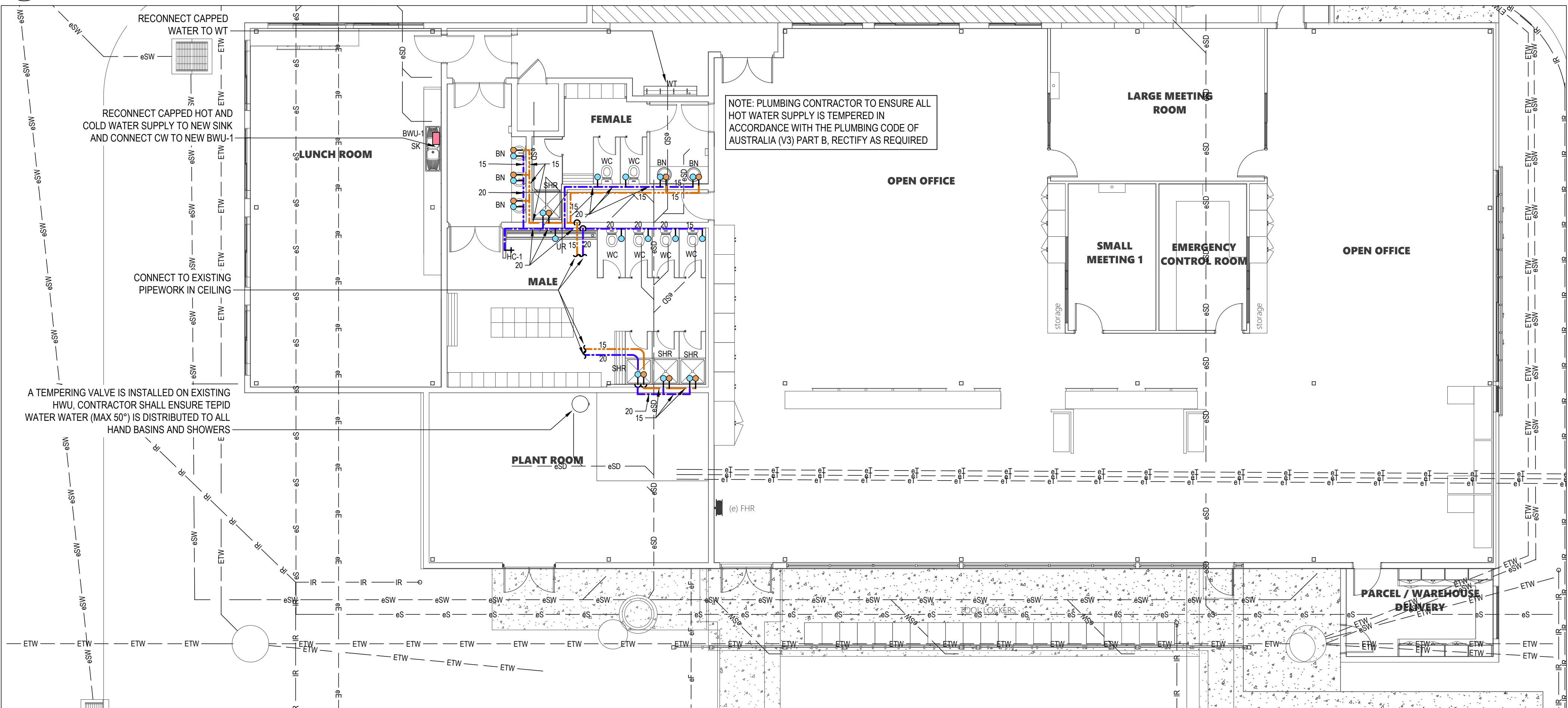
2 Proposed Floor Plan - Water Scale: 1:100 @ A1
