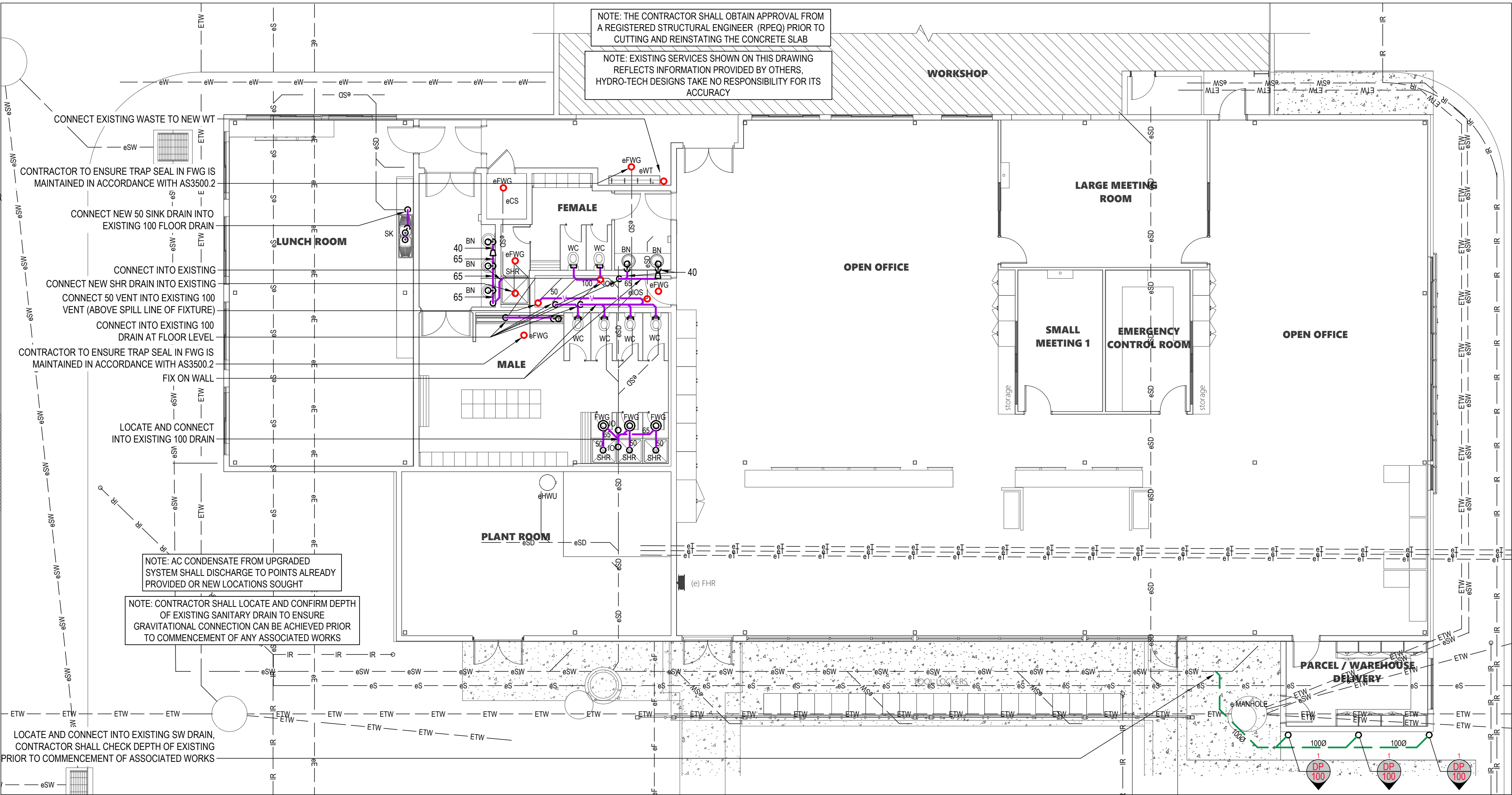
1 Proposed Floor Plan - Drainage Scale: 1:100 @ A1
